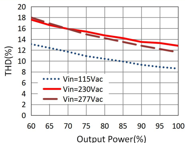
THD VS Output Power
