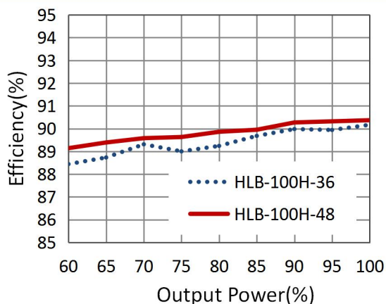
Efficiency VS Output Power
